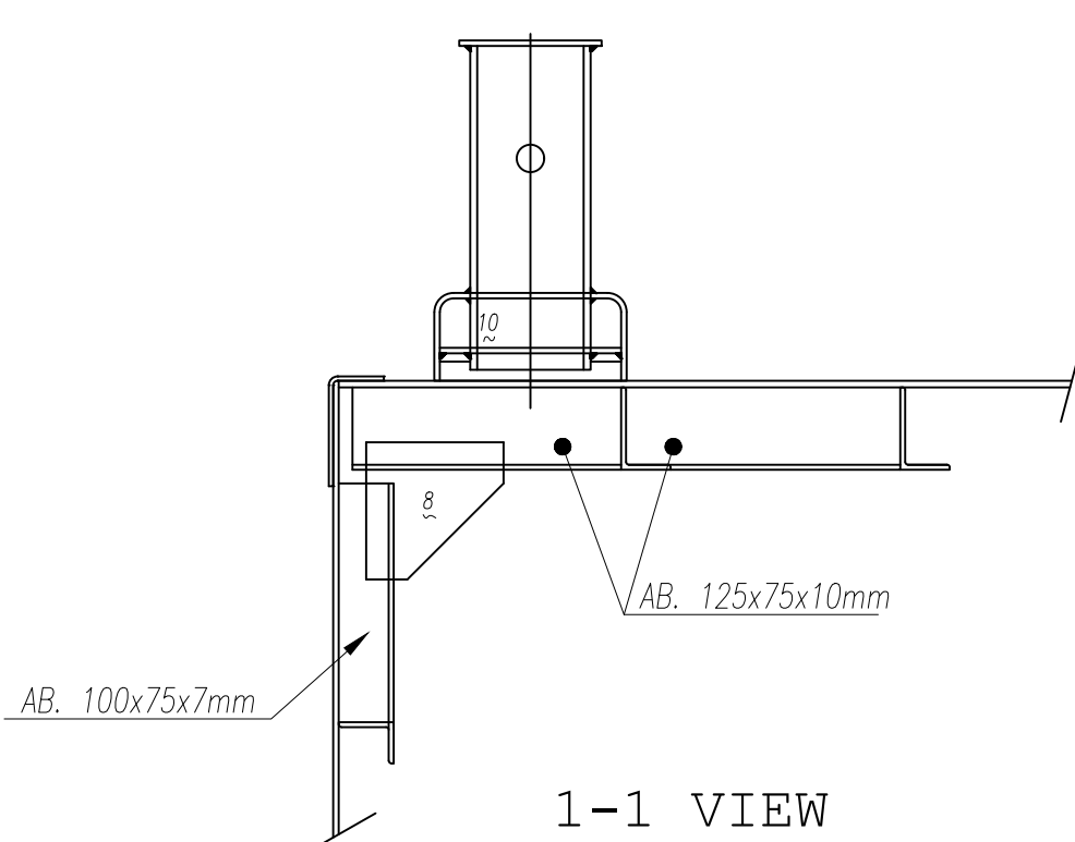
1-1 VIEW
