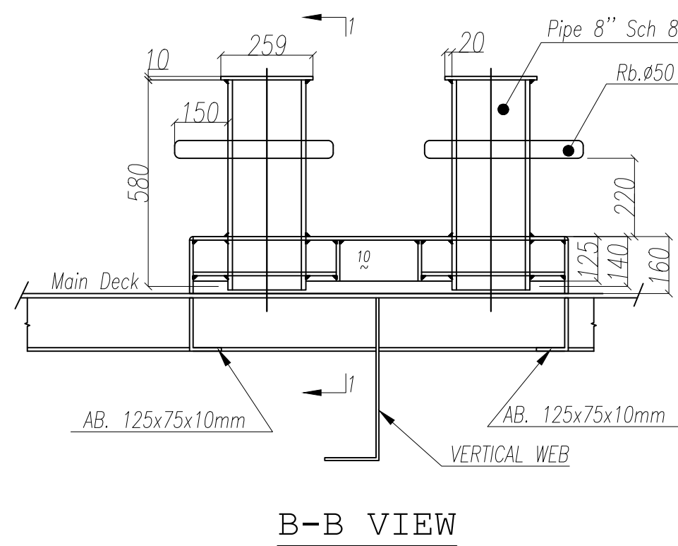
B-B VIEW
